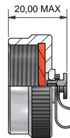
100P1240-16-1-C-EO EYELET ONLY VERSION (NO LANYARD)
